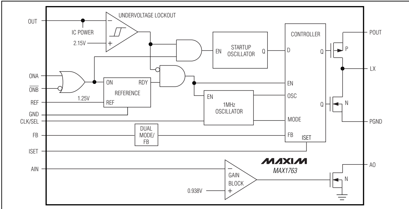
Figure 1. Functional Diagram
